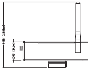
RIGHT VIEW
